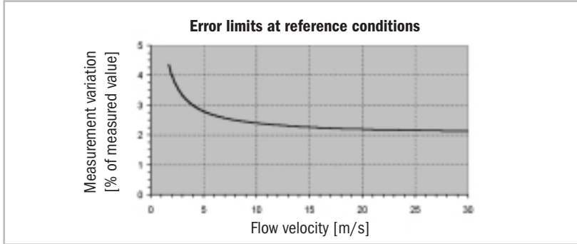
Fig. 22: Dual-beam ultrasonic flowmeter, errors of measurement
