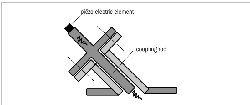
Fig. 18: Schematic sketch of an ultrasonic high-temperature/high-pressure sensor
