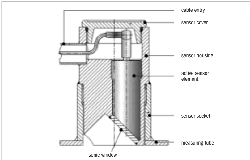
Fig. 16: The active sensor element is replaceable at process conditions
