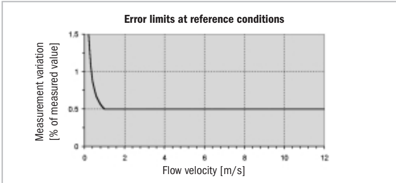
Fig. 17: Error limits of a dual-beam ultrasonic flowmeter for liquids
