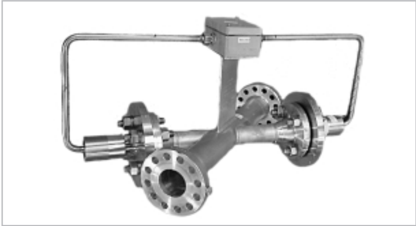
Fig. 19: High-temperature version with heating jacket for liquid or steam tracing
