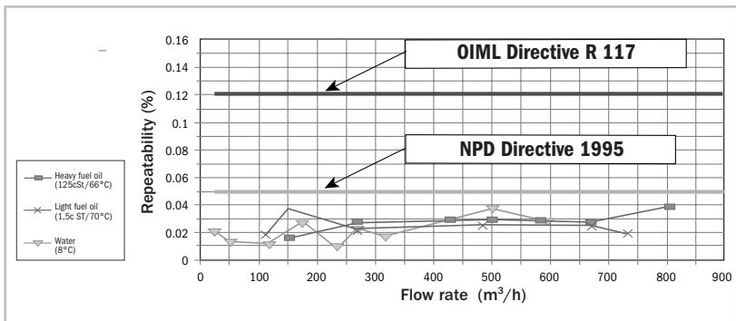
Fig. 28: ALTOSONIC V ultrasonic volumeter: repeatability: < 0.05% of the measured value!
